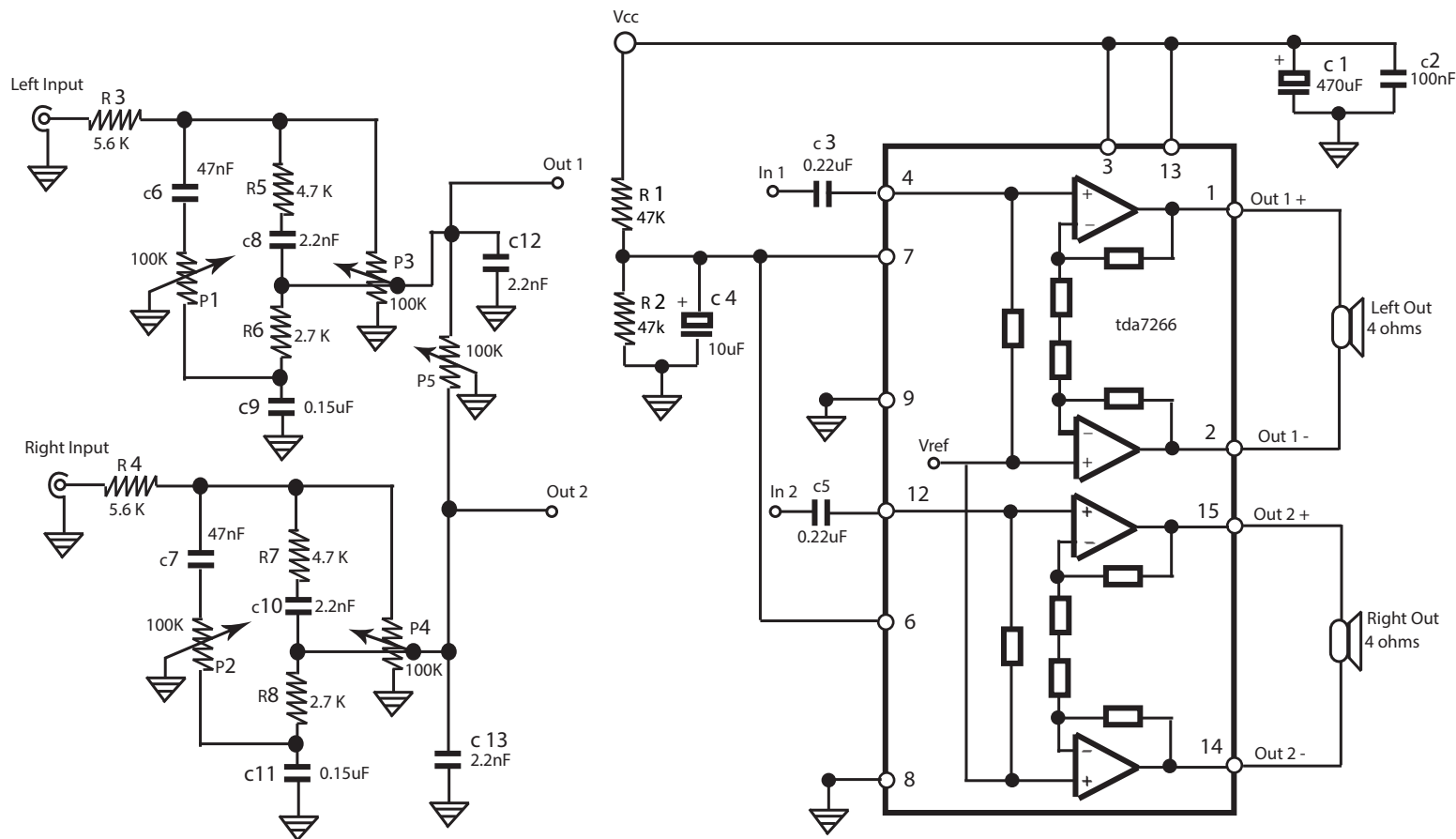
7 by 7 power amp using TDA7266 Holmes 1/4/18
